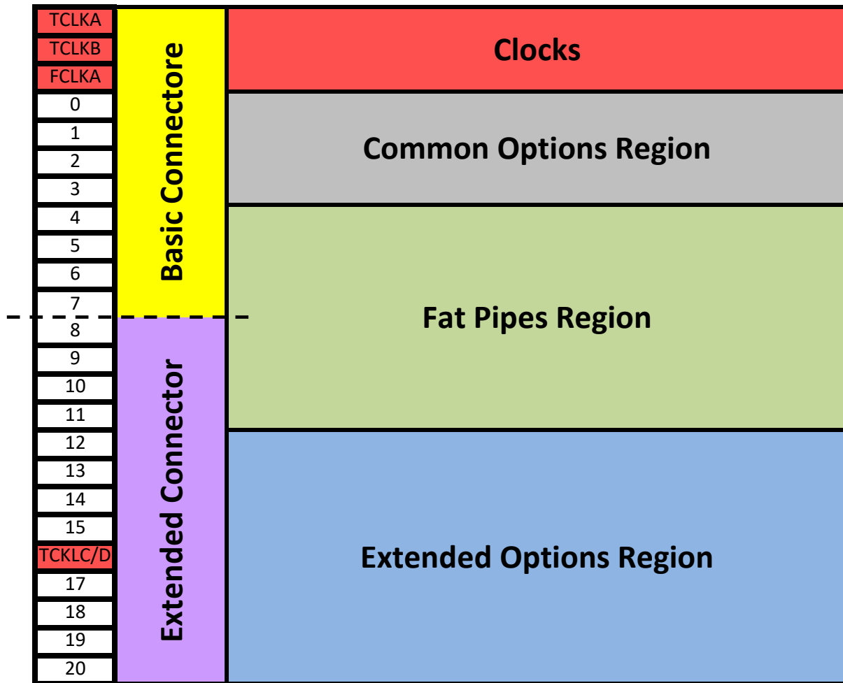
AMC Port mapping guidance per PICMG® AMC.0 R2.0 Dec 28,2006
